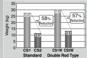
CS1→CS2 Weight Comparison (Basic Type \varnothing 160-100st )
